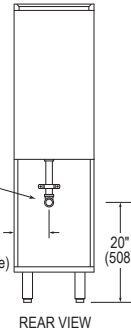
REAR VIEW
